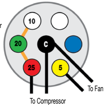
Illustration 5mfd Fan 55mfd Compressor
